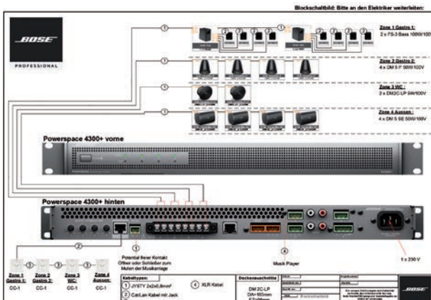
Preparation of detailed wiring diagrams by Bose Professional partners.
